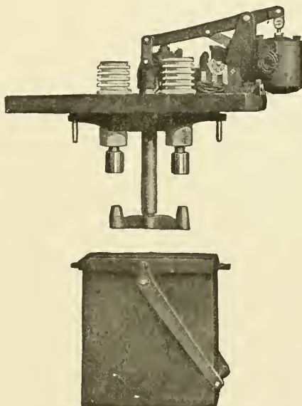
Fig. 154. Single-Pole Westinghouse Type E Electrically-Operated Oil Circuit Breaker
